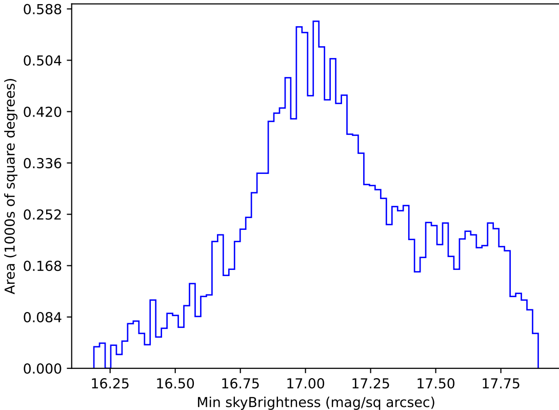
smc_lmc_v3.3_10yrs WFD y band: Min skyBrightness
