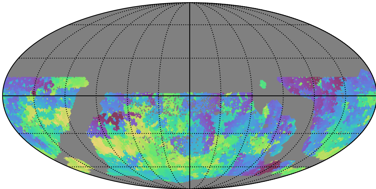
smc_lmc_v3.3_10yrs WFD u band: Min skyBrightness
