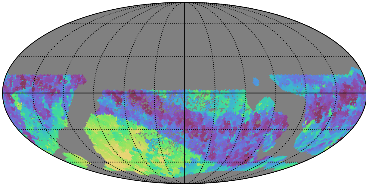
smc_lmc_v3.3_10yrs WFD i band: Min skyBrightness
