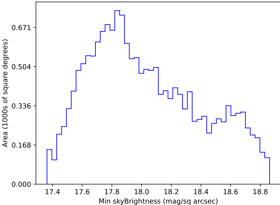
smc_lmc_v3.3_10yrs WFD i band: Min skyBrightness
