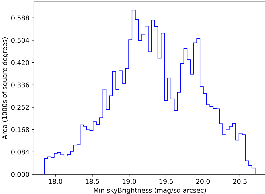
smc_lmc_v3.3_10yrs WFD g band: Min skyBrightness
