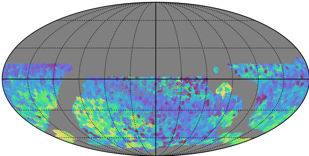
smc_lmc_v3.3_10yrs WFD all bands: Min skyBrightness
