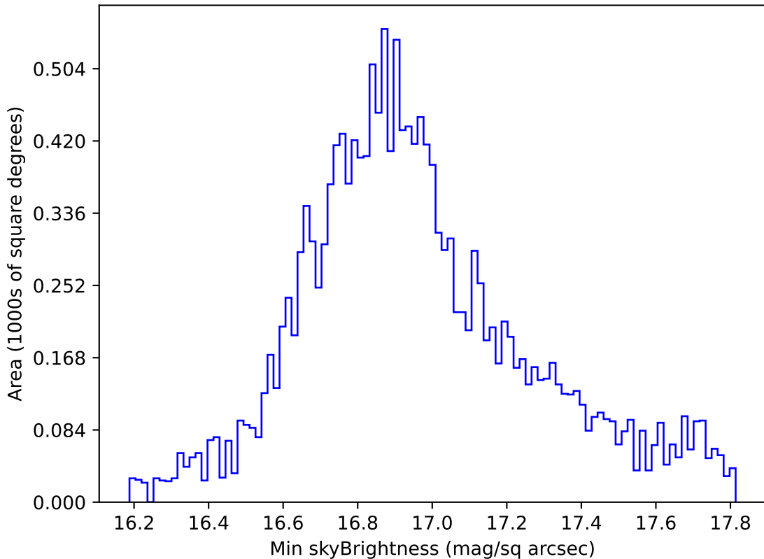
smc_lmc_v3.3_10yrs WFD all bands: Min skyBrightness
