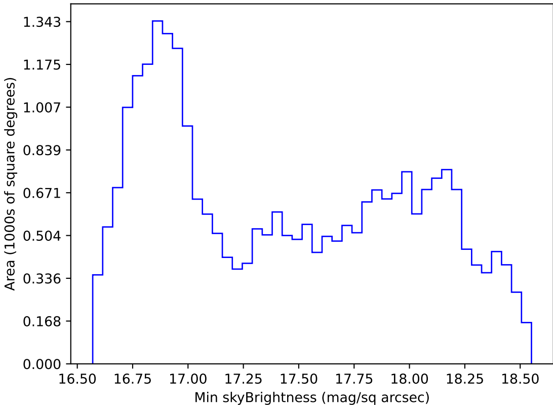
smc_lmc_v3.3_10yrs All sky z band: Min skyBrightness
