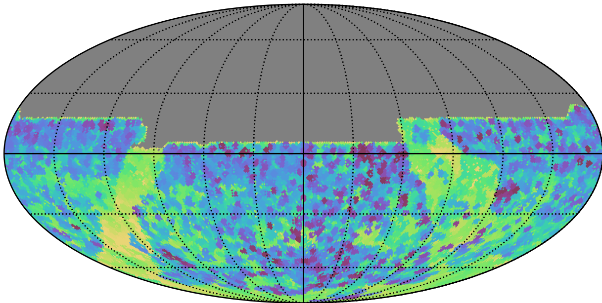
smc_lmc_v3.3_10yrs All sky y band: Min skyBrightness
