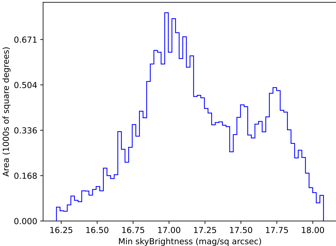
smc_lmc_v3.3_10yrs All sky y band: Min skyBrightness
