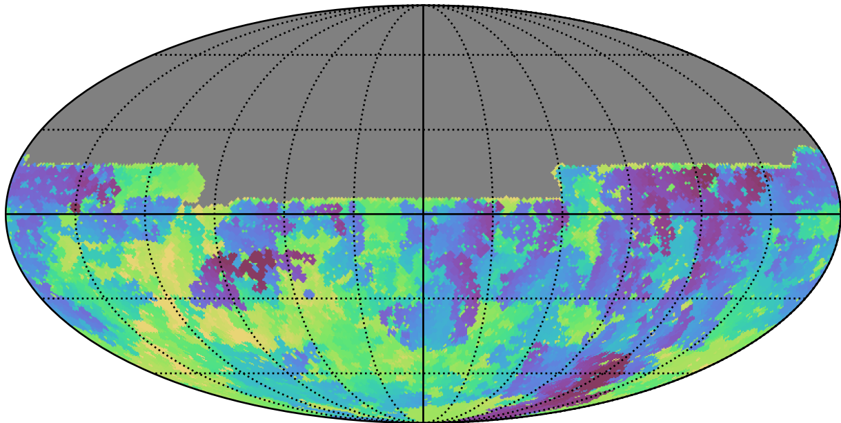
smc_lmc_v3.3_10yrs All sky u band: Min skyBrightness
