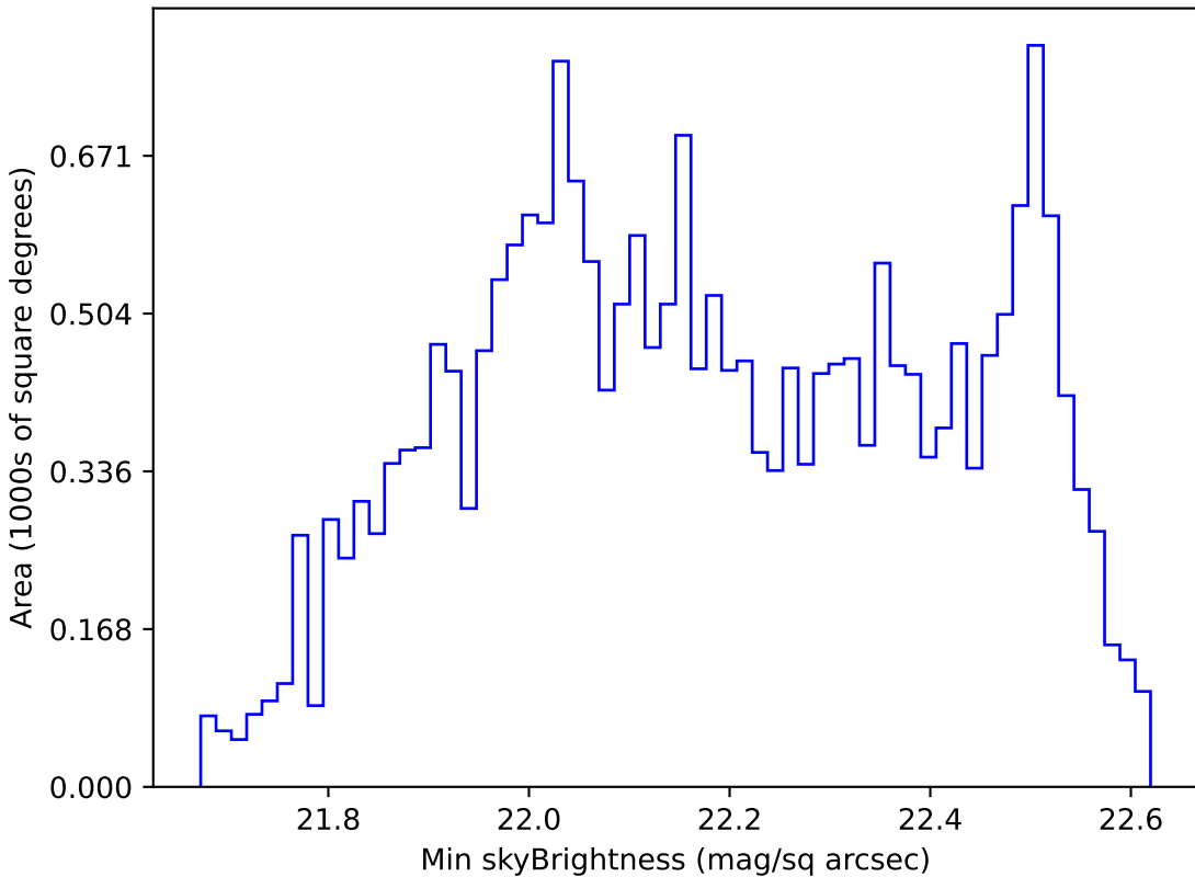
smc_lmc_v3.3_10yrs All sky u band: Min skyBrightness
