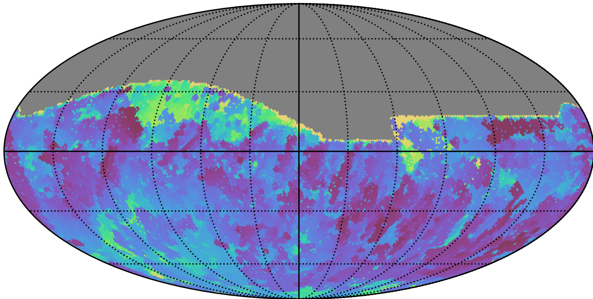
smc_lmc_v3.3_10yrs All sky r band: Min skyBrightness
