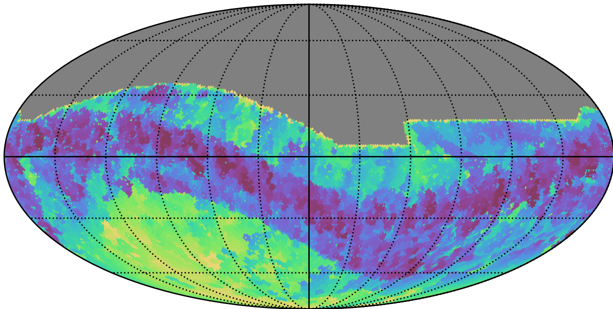
smc_lmc_v3.3_10yrs All sky i band: Min skyBrightness
