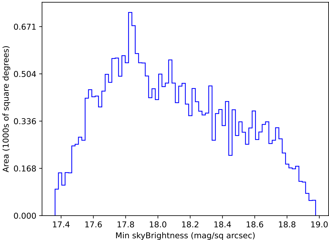
smc_lmc_v3.3_10yrs All sky i band: Min skyBrightness
