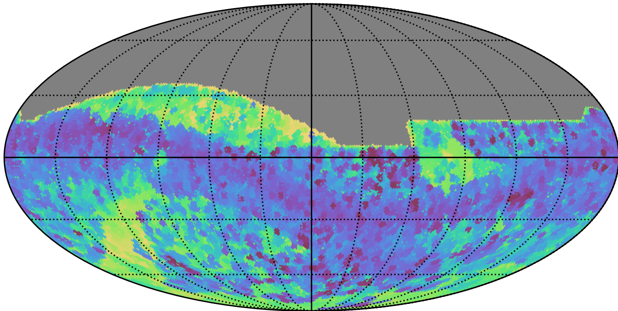
smc_lmc_v3.3_10yrs All sky all bands: Min skyBrightness
