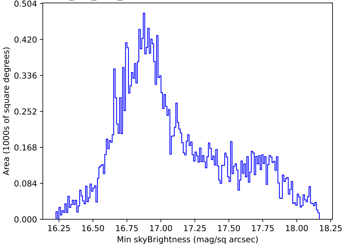
smc_lmc_v3.3_10yrs All sky all bands: Min skyBrightness
