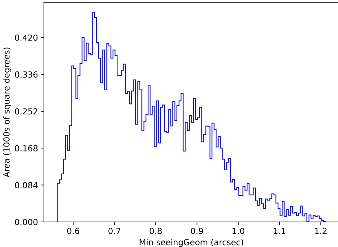
smc_lmc_v3.3_10yrs Yr 1 u band: Min seeingGeom
