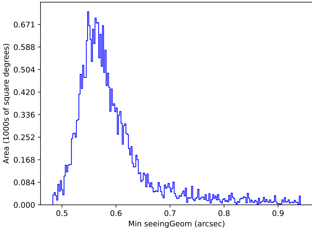
smc_Imc_v3.3_10yrs Yr 1 all bands: Min seeingGeom
