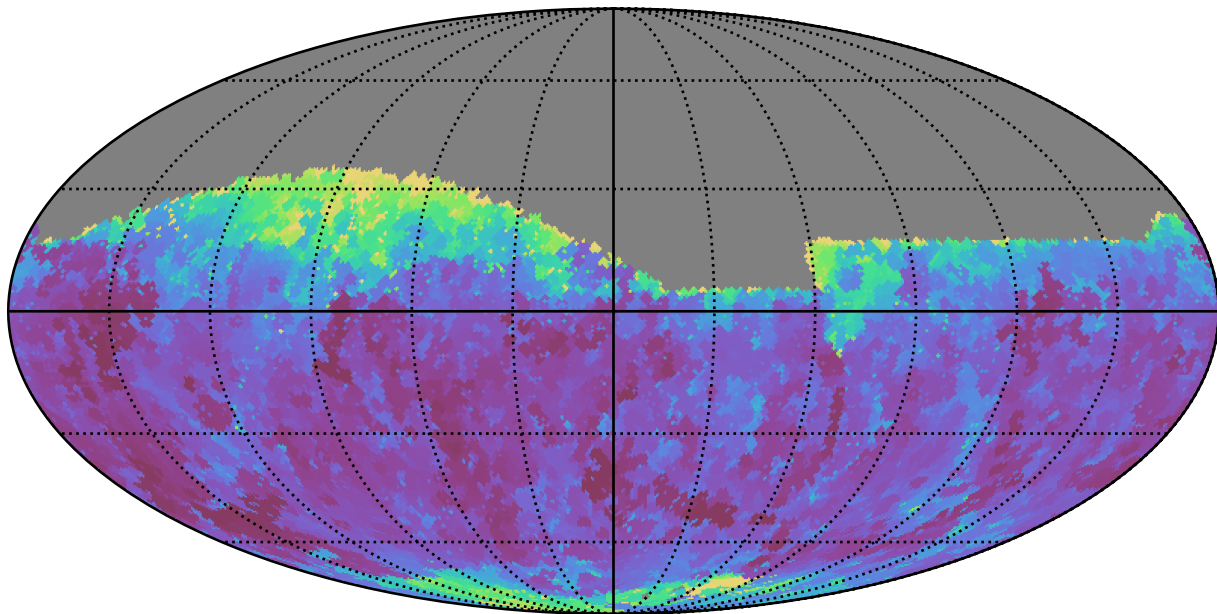
smc_lmc_v3.3_10yrs Yr 1 z band: Min seeingEff
