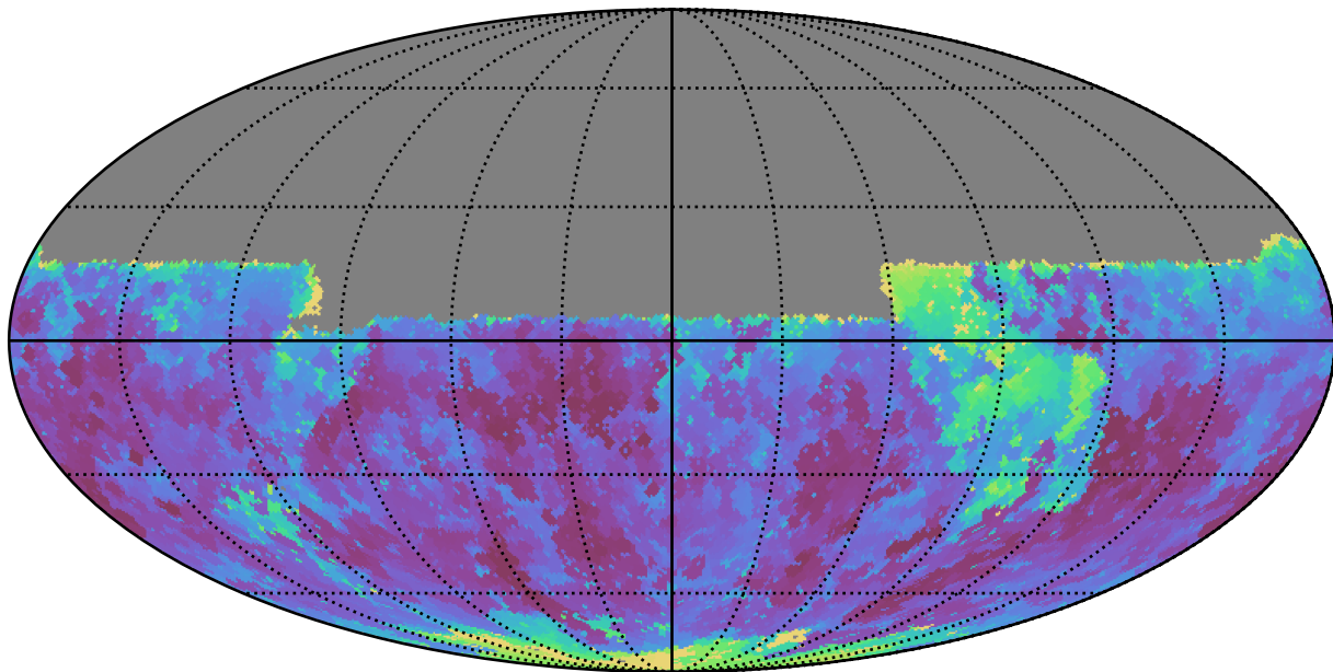
smc_lmc_v3.3_10yrs Yr 1 y band: Min seeingEff
