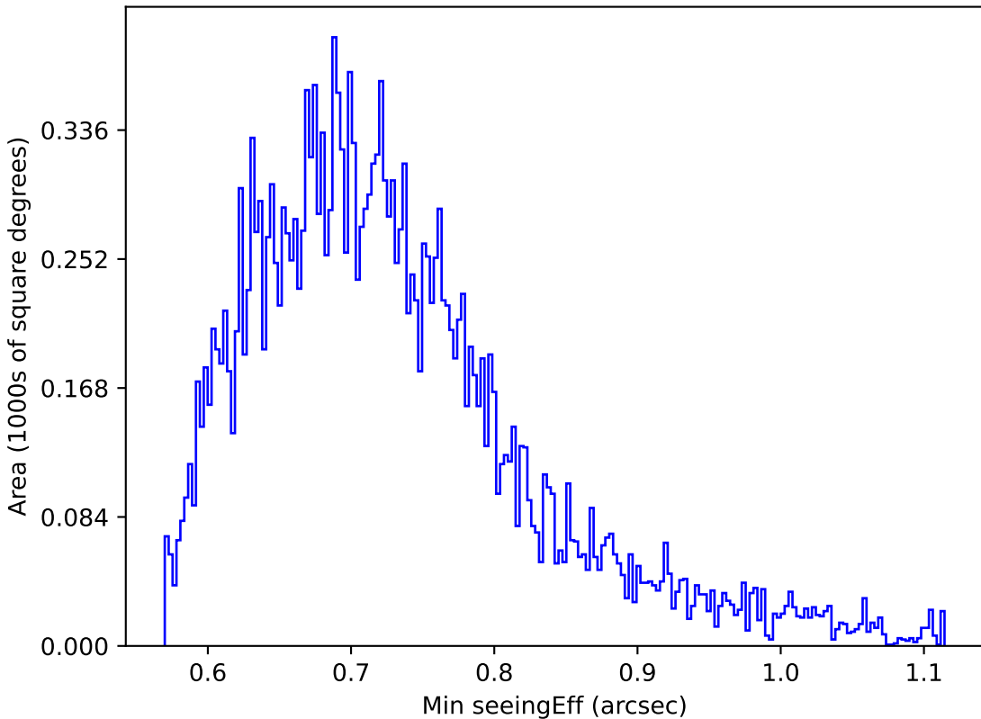
smc_lmc_v3.3_10yrs Yr 1 y band: Min seeingEff
