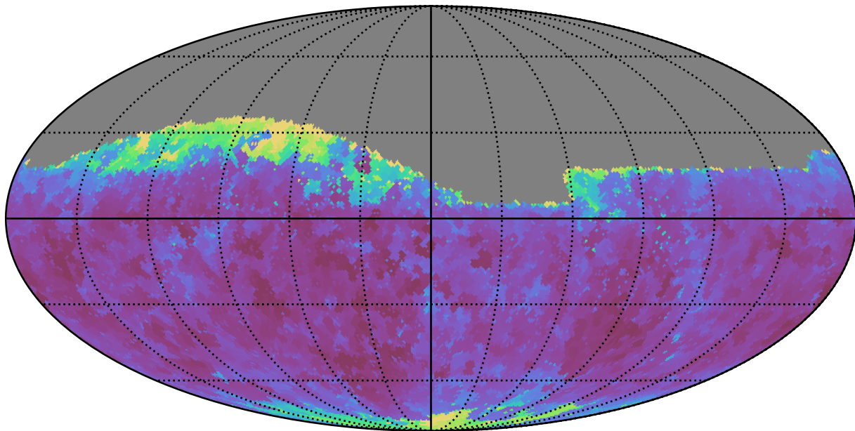
smc_lmc_v3.3_10yrs Yr 1 r band: Min seeingEff
