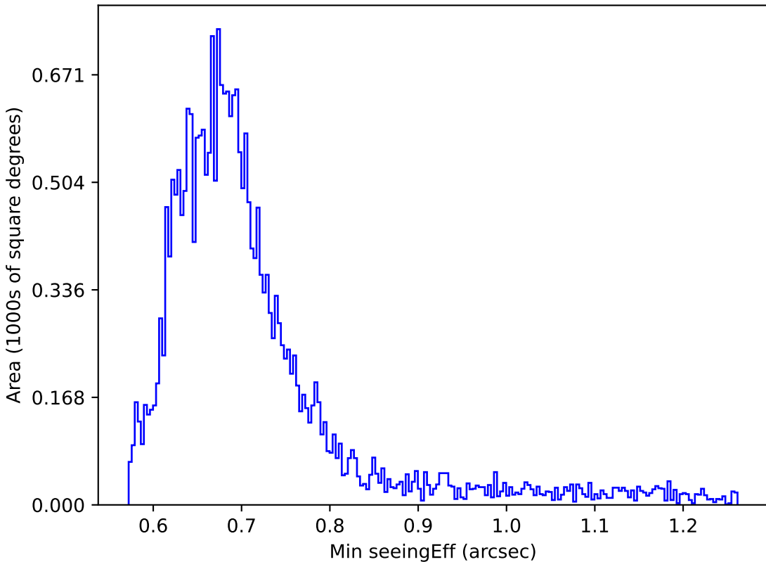
smc_lmc_v3.3_10yrs Yr 1 r band: Min seeingEff
