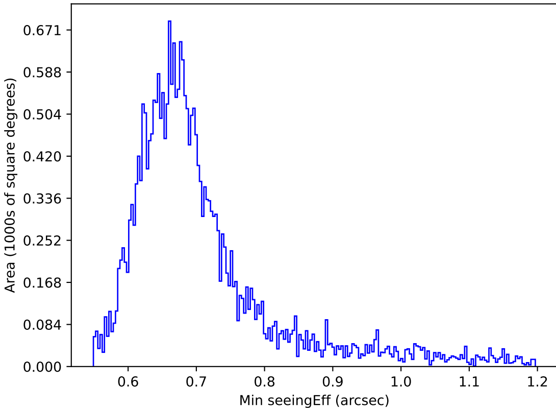
smc_lmc_v3.3_10yrs Yr 1 i band: Min seeingEff
