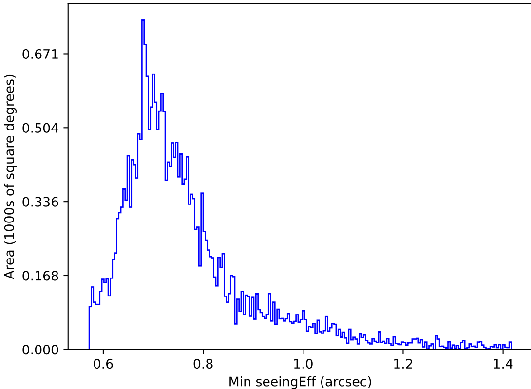
smc_lmc_v3.3_10yrs Yr 1 g band: Min seeingEff
