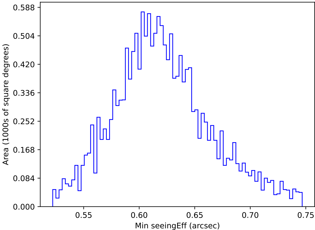
smc_lmc_v3.3_10yrs WFD z band: Min seeingEff
