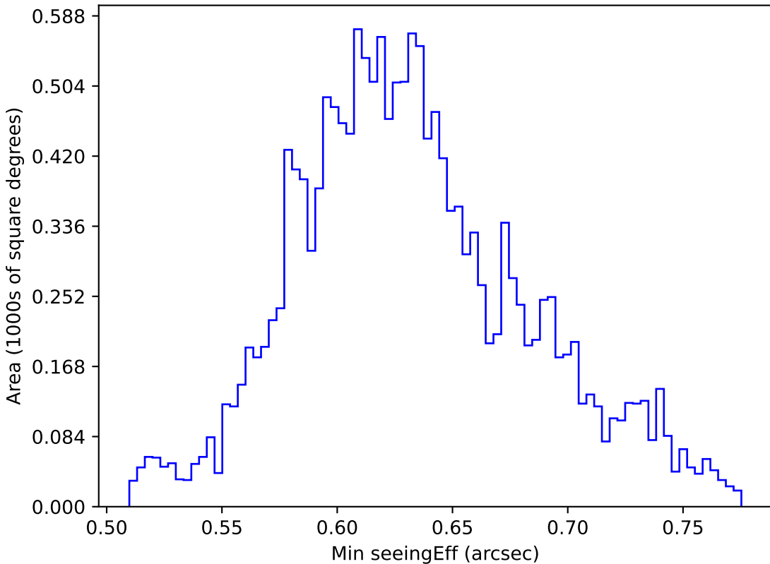
smc_lmc_v3.3_10yrs WFD y band: Min seeingEff
