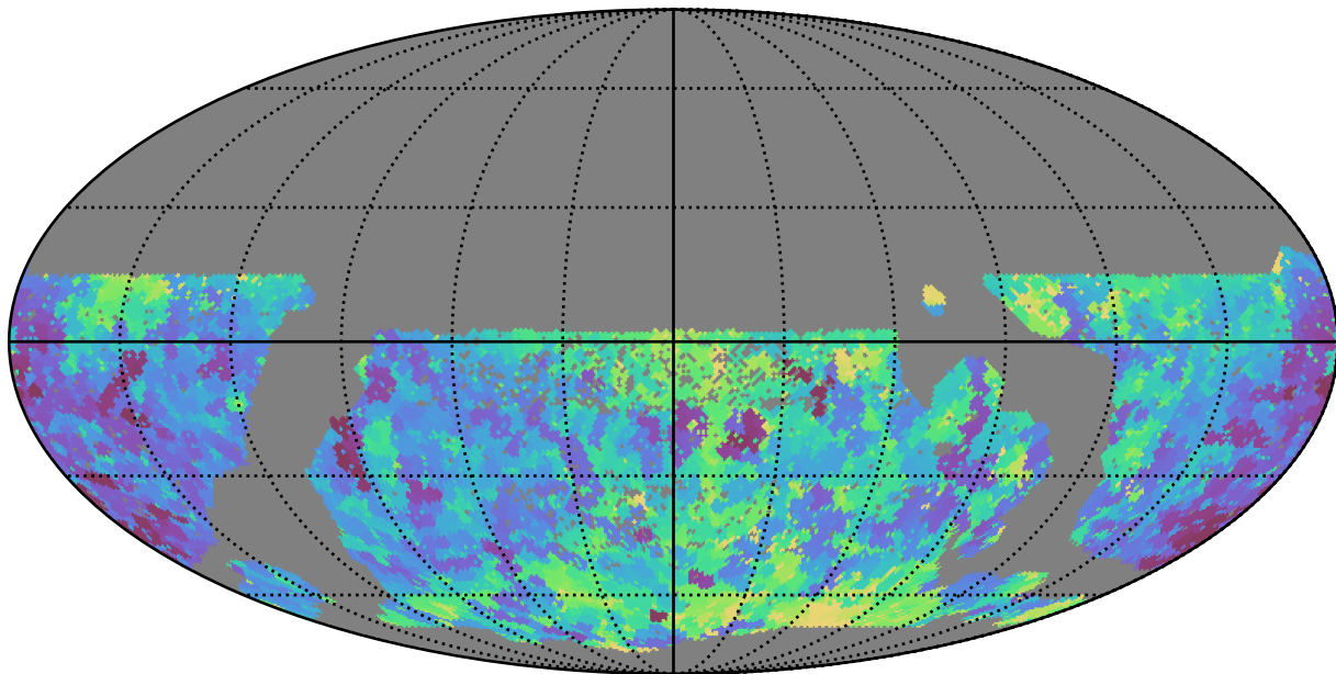
smc_lmc_v3.3_10yrs WFD u band: Min seeingEff
