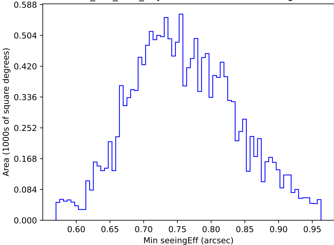
smc_lmc_v3.3_10yrs WFD u band: Min seeingEff
