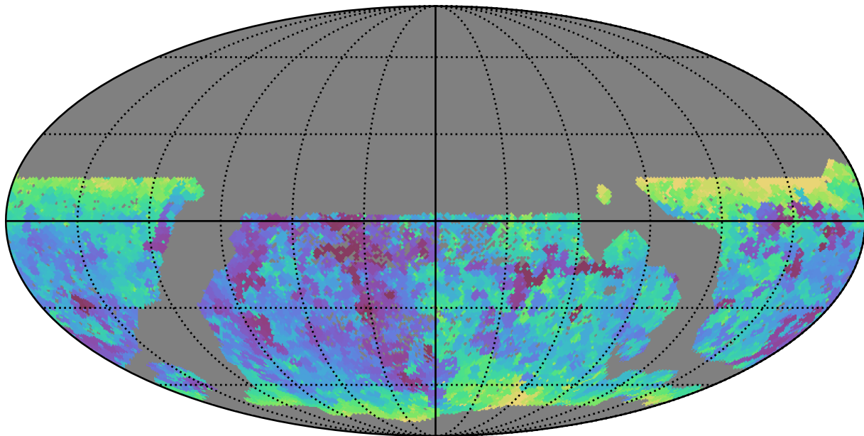
smc_lmc_v3.3_10yrs WFD r band: Min seeingEff
