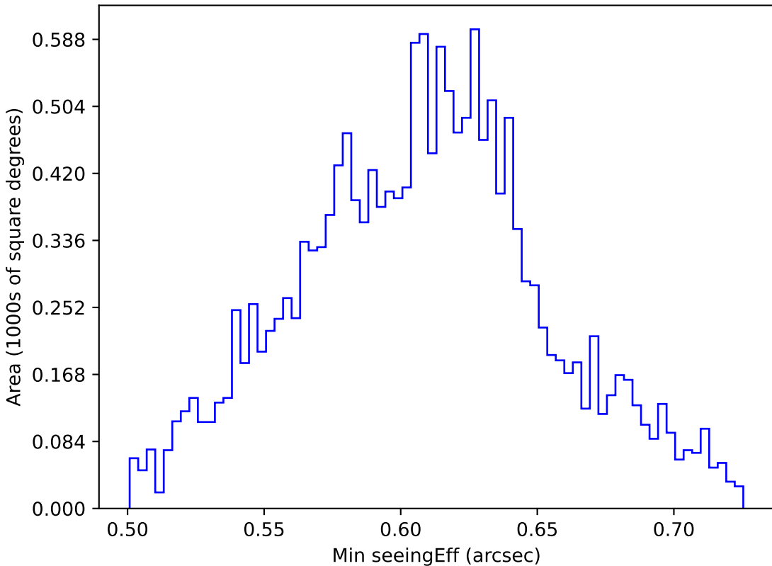
smc_lmc_v3.3_10yrs WFD r band: Min seeingEff
