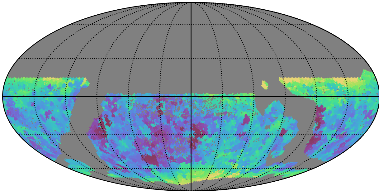
smc_lmc_v3.3_10yrs WFD i band: Min seeingEff
