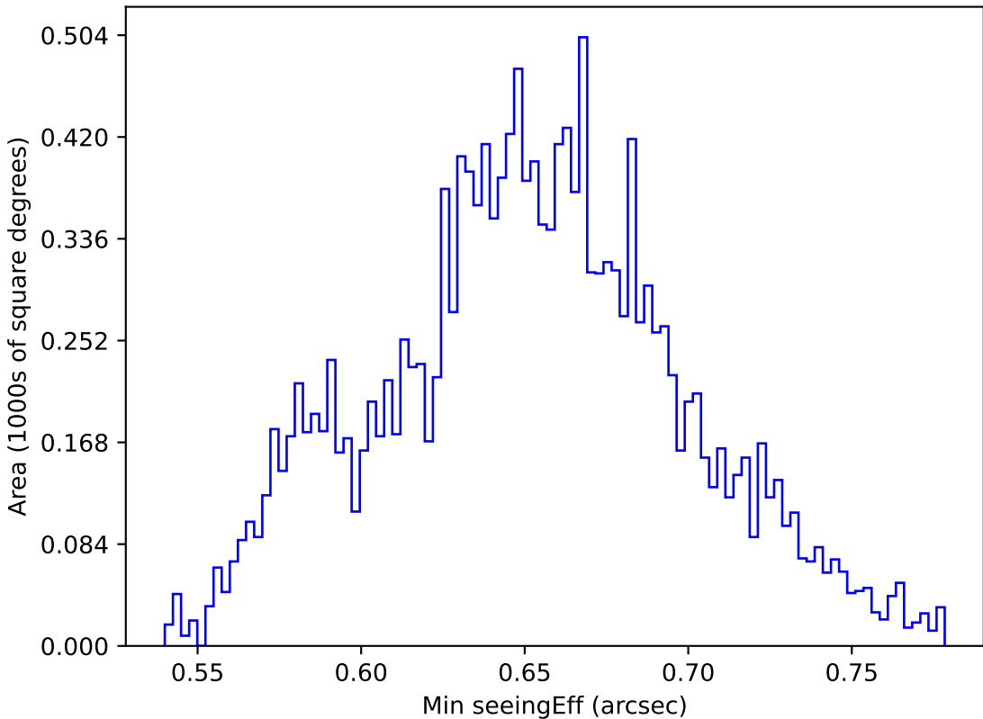
smc_lmc_v3.3_10yrs WFD g band: Min seeingEff
