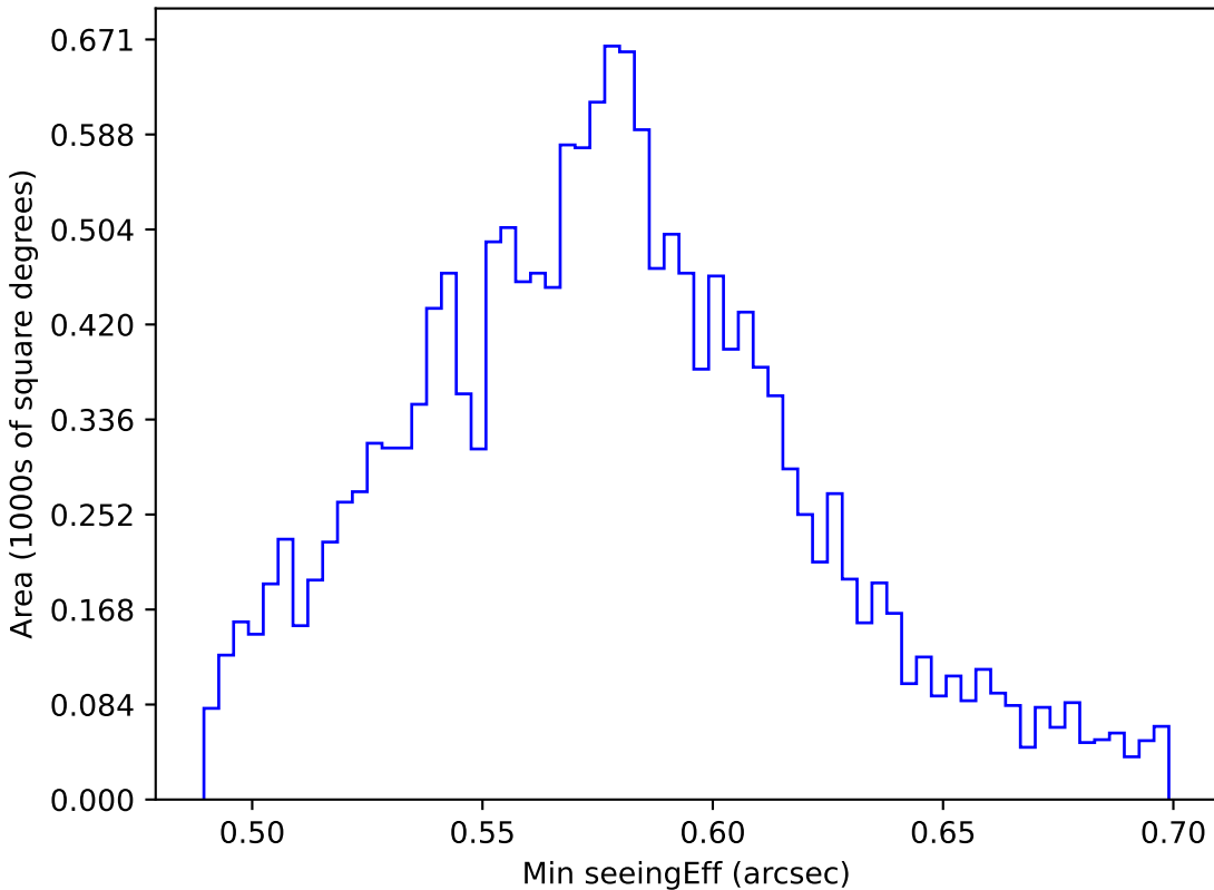
smc_lmc_v3.3_10yrs WFD all bands: Min seeingEff
