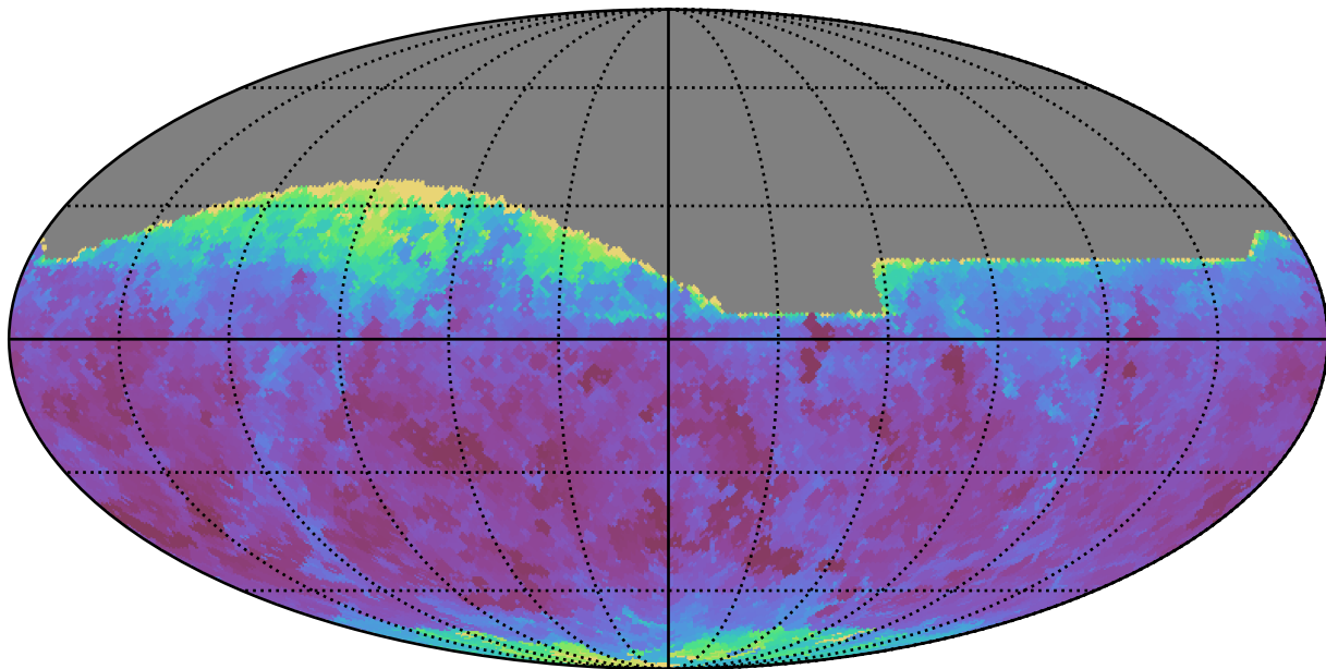
smc_lmc_v3.3_10yrs All sky z band: Min seeingEff
