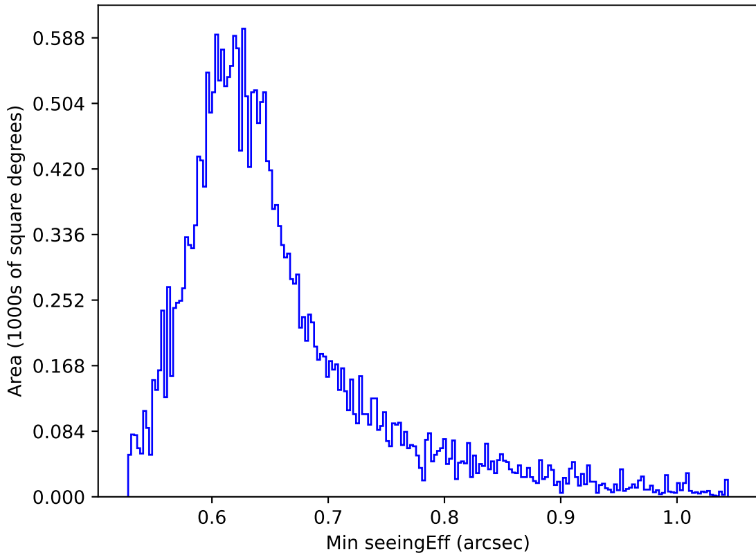
smc_lmc_v3.3_10yrs All sky z band: Min seeingEff
