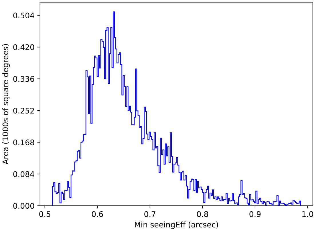
smc_lmc_v3.3_10yrs All sky y band: Min seeingEff
