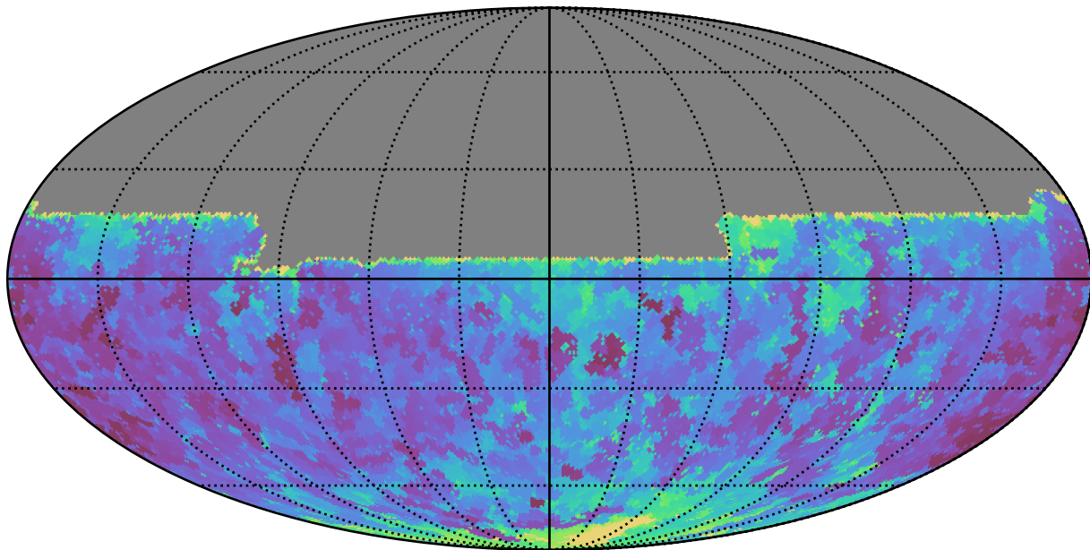
smc_lmc_v3.3_10yrs All sky u band: Min seeingEff
