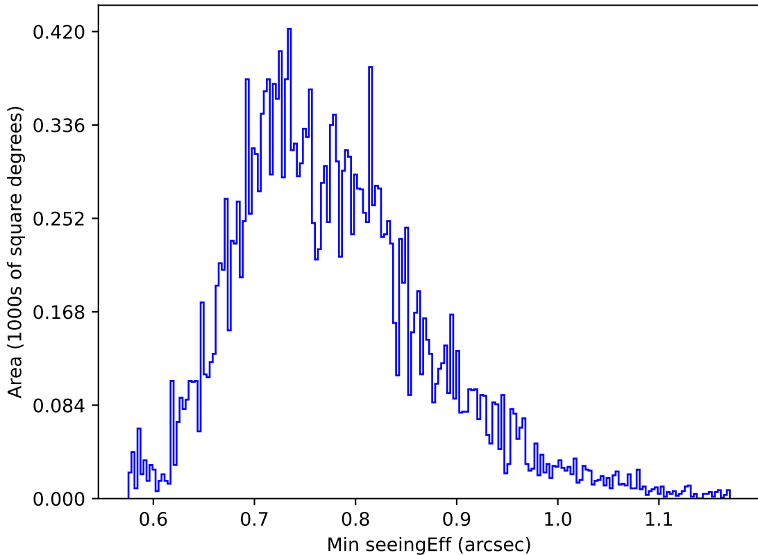
smc_lmc_v3.3_10yrs All sky u band: Min seeingEff
