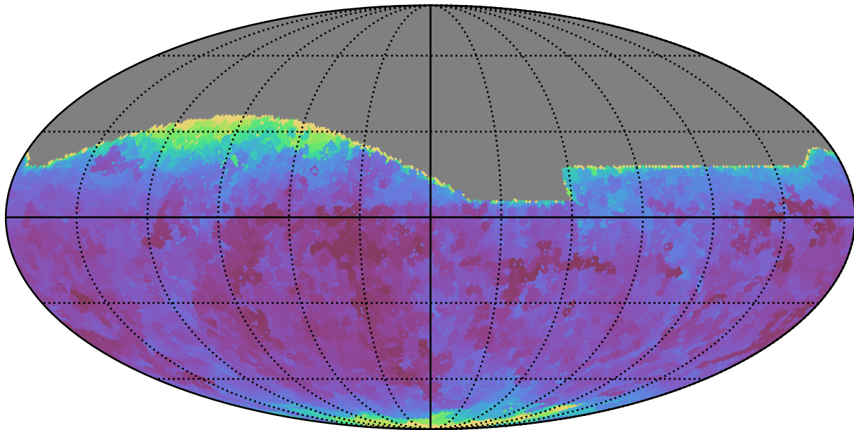
smc_lmc_v3.3_10yrs All sky r band: Min seeingEff
