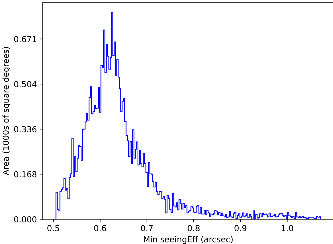
smc_lmc_v3.3_10yrs All sky r band: Min seeingEff
