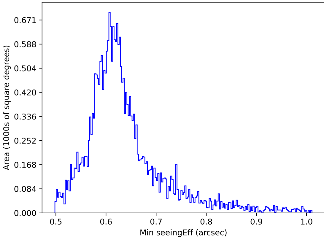
smc_lmc_v3.3_10yrs All sky i band: Min seeingEff
