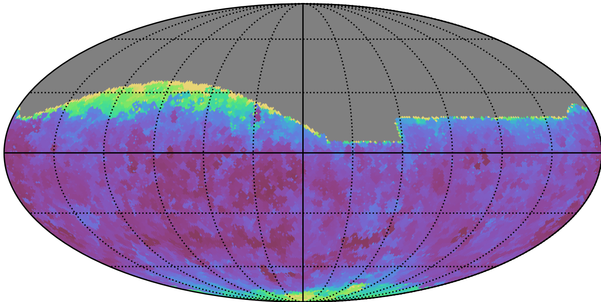
smc_lmc_v3.3_10yrs All sky g band: Min seeingEff
