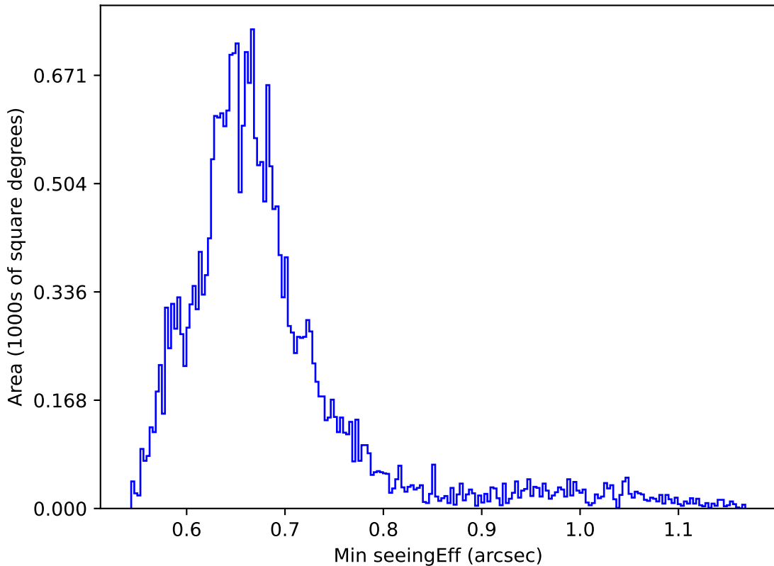
smc_lmc_v3.3_10yrs All sky g band: Min seeingEff
