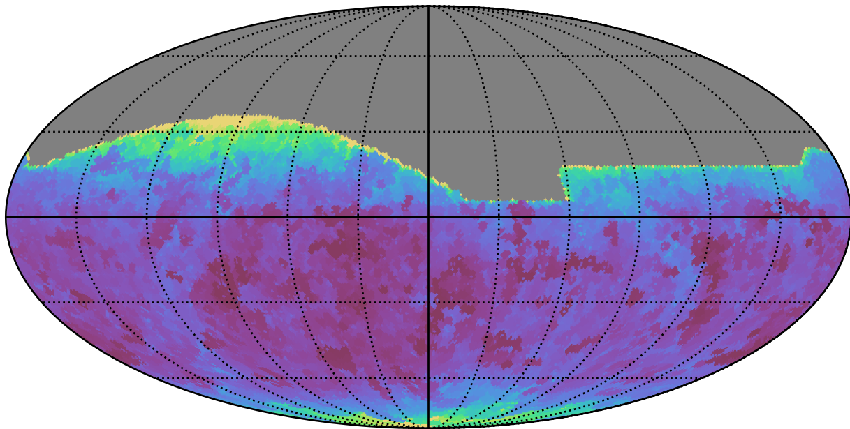
smc_lmc_v3.3_10yrs All sky all bands: Min seeingEff
