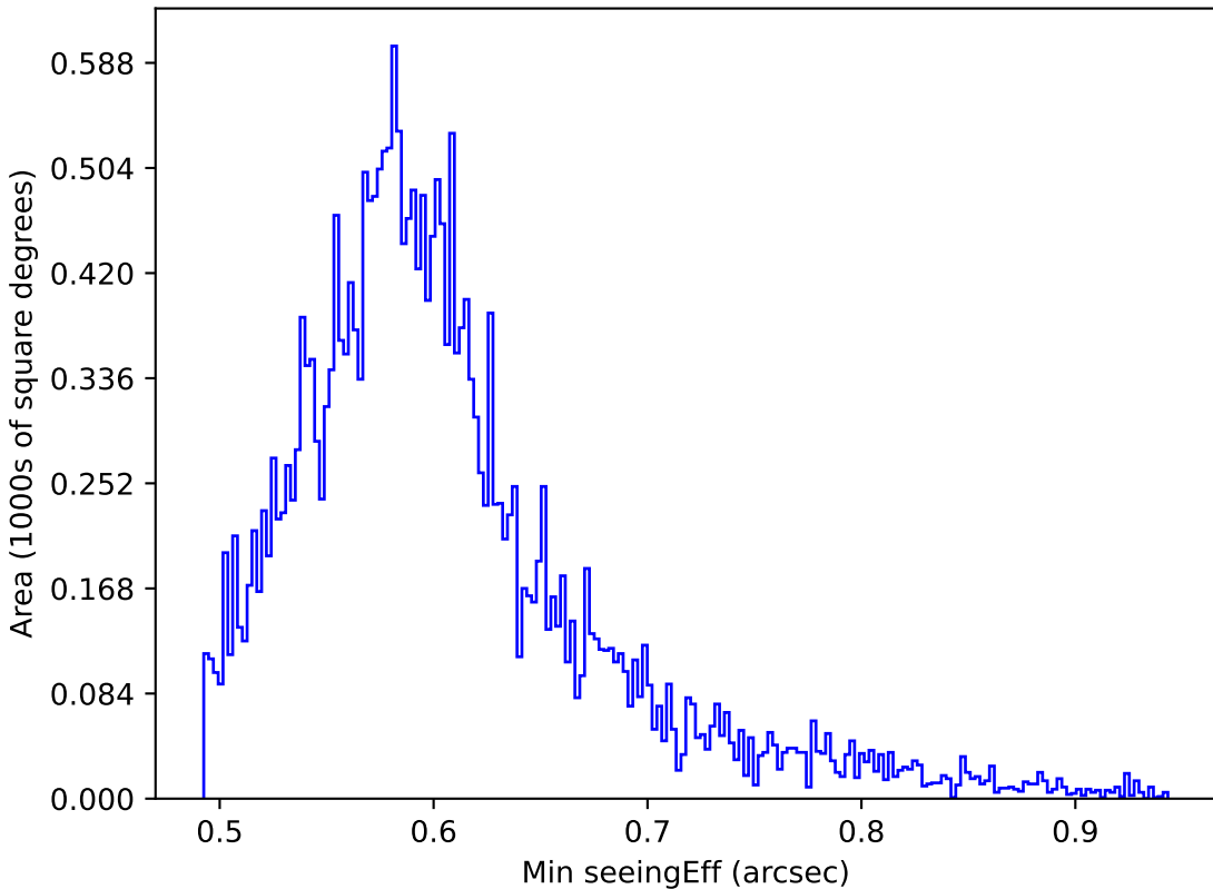
smc_lmc_v3.3_10yrs All sky all bands: Min seeingEff
