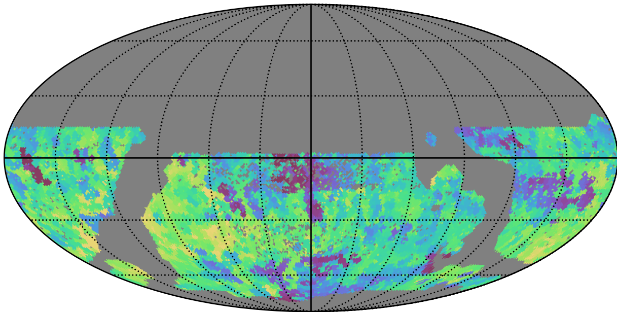
smc_lmc_v3.3_10yrs WFD z band: Min saturation_mag
