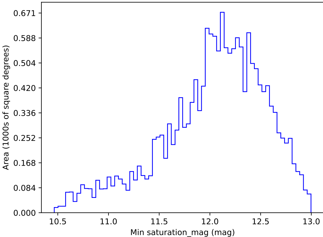
smc_lmc_v3.3_10yrs WFD z band: Min saturation_mag
