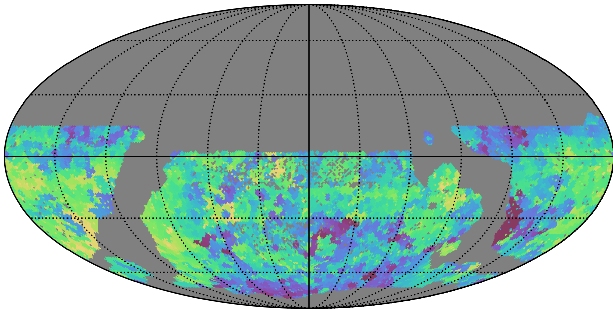
smc_lmc_v3.3_10yrs WFD u band: Min saturation_mag
